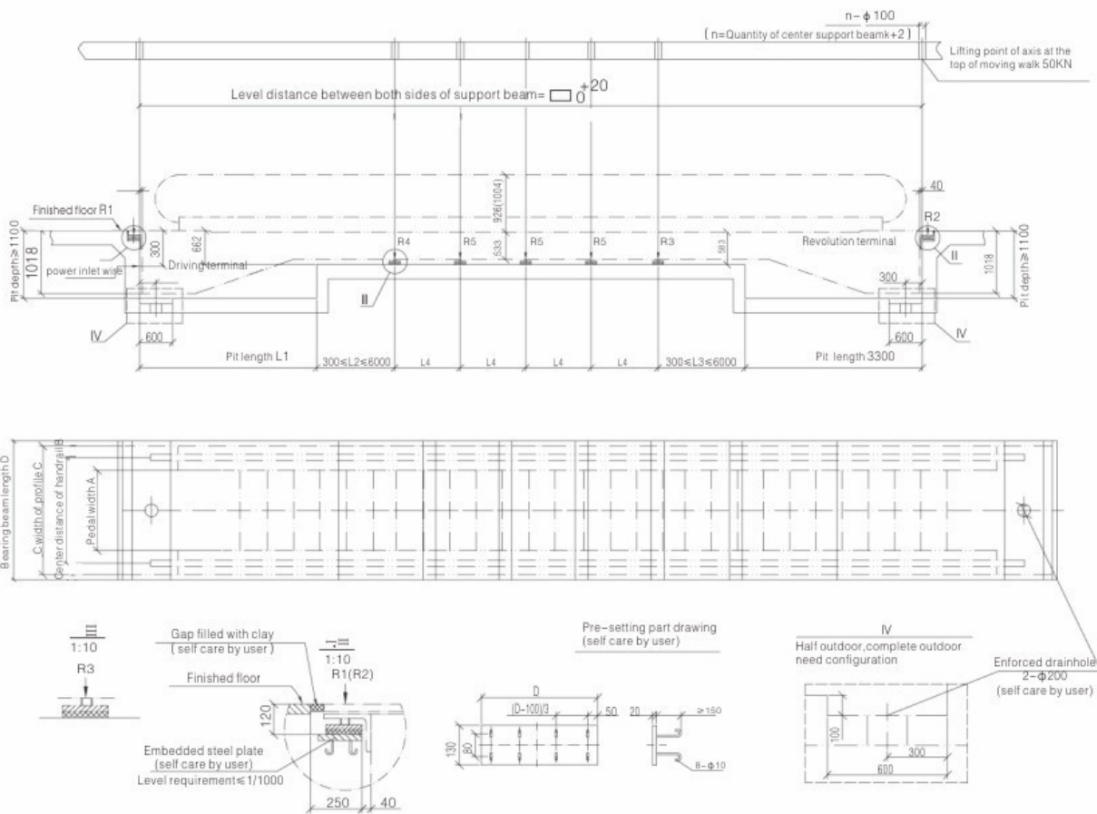
0° Moving walk construction layout drawing
