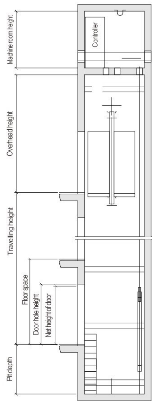
Shaft elevation
