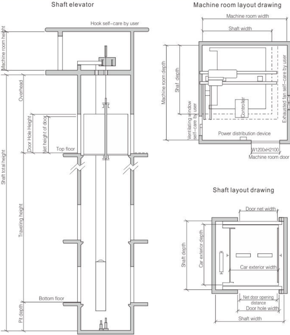
Freight elevator specifications
