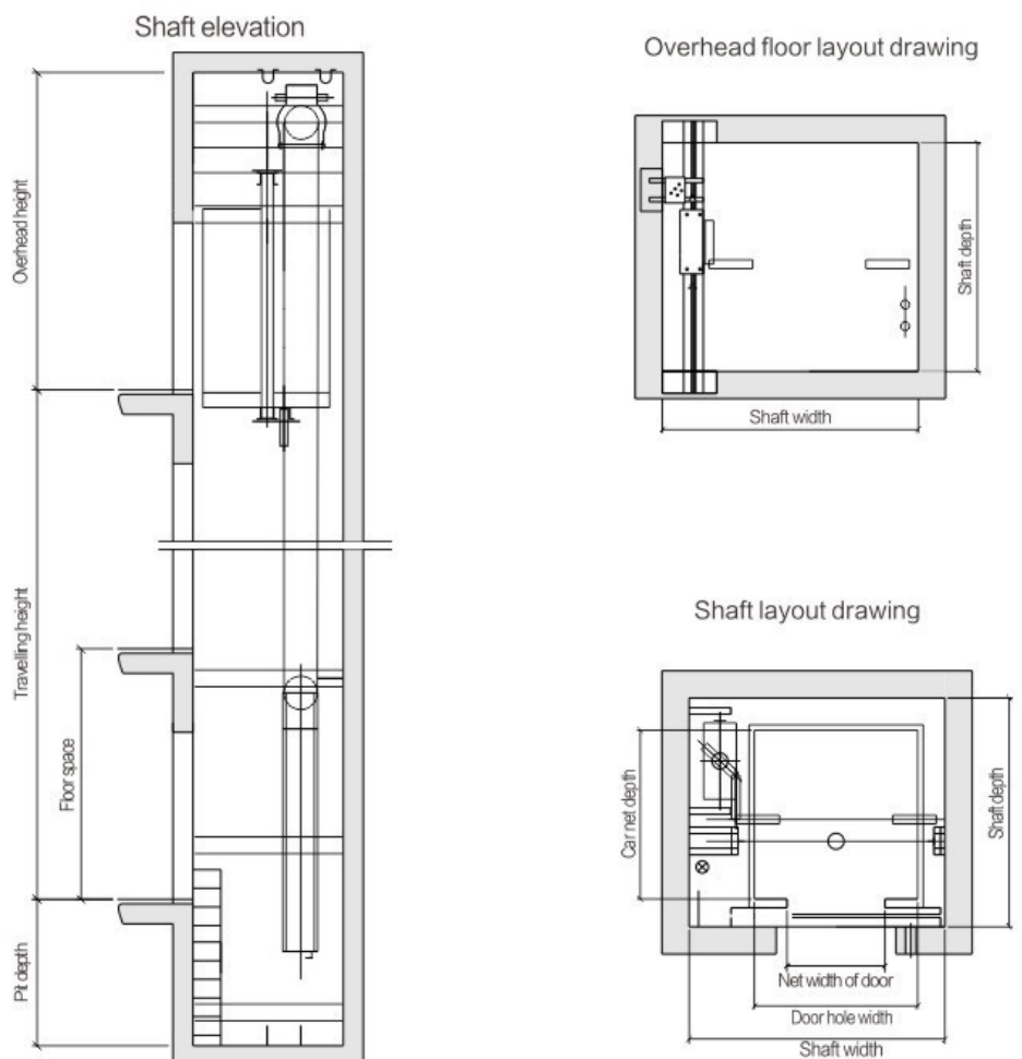
Square machine room / Machine roomless elevator specifications
