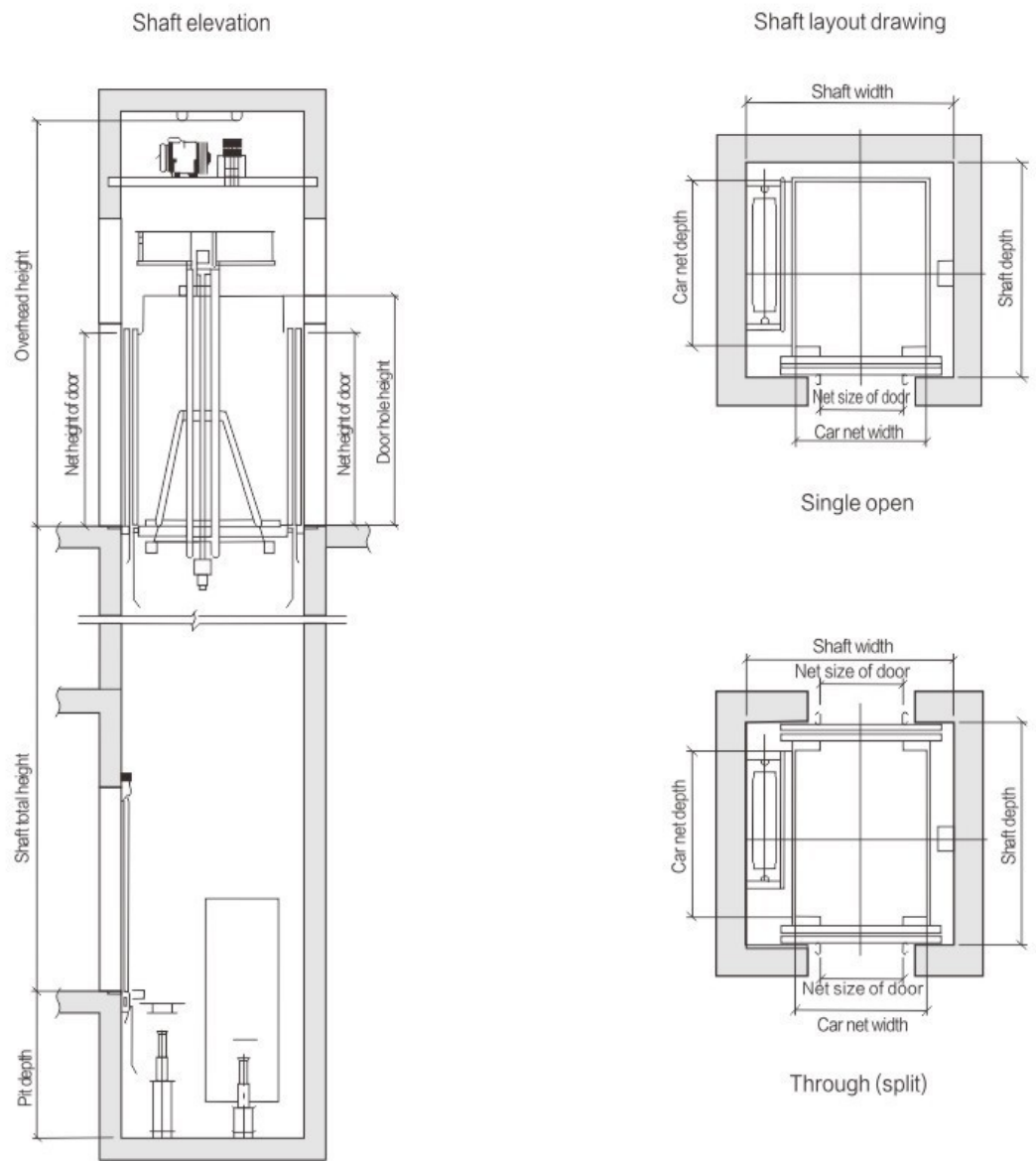
Steel structure elevator specifications
